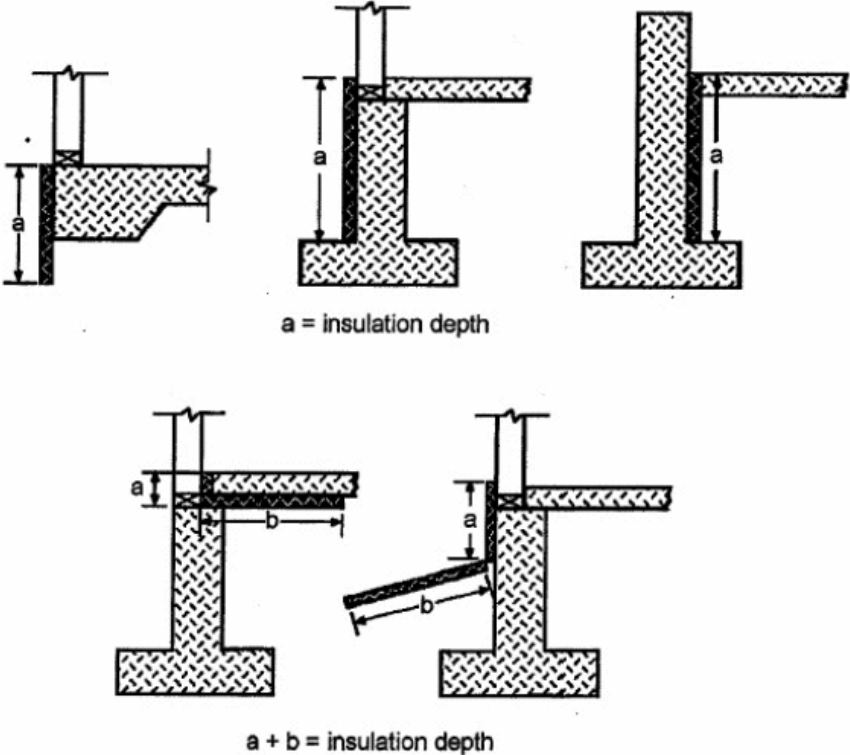
Figure 402.2.7 SLAB EDGE INSULATION METHODS
